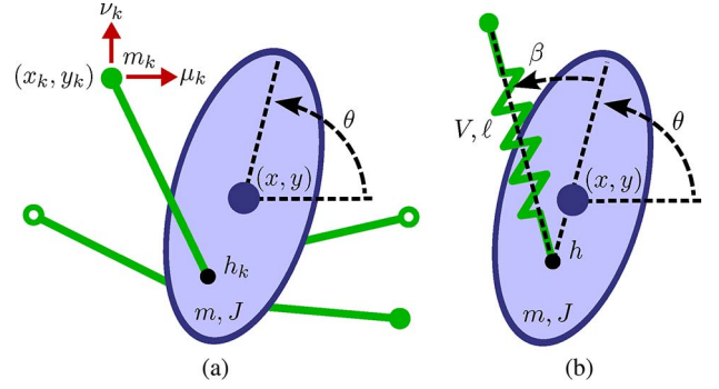
Fig. 4. Lateral-plane models for locomotion described in Section IV-B. (a) Polyped with n = 4 legs, leg k annotated; (b) Lateral Leg-Spring (LLS) [17].
