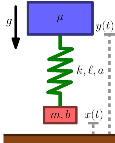
Fig. 3. Schematic of vertical hopper. Two masses m and \mu , constrained to move vertically above a ground plane in a gravitational field with magnitude g , are connected by a linear spring with stiffness k and nominal length \ell . The lower mass experiences viscous drag proportional to velocity with constant b when it is in the air, and impacts plastically with the ground (i.e., it is not permitted to penetrate the ground and its velocity is instantaneously set to zero whenever a collision occurs). When the lower mass is in contact with the ground, the spring stiffness is multiplied by a constant a > 1 .
