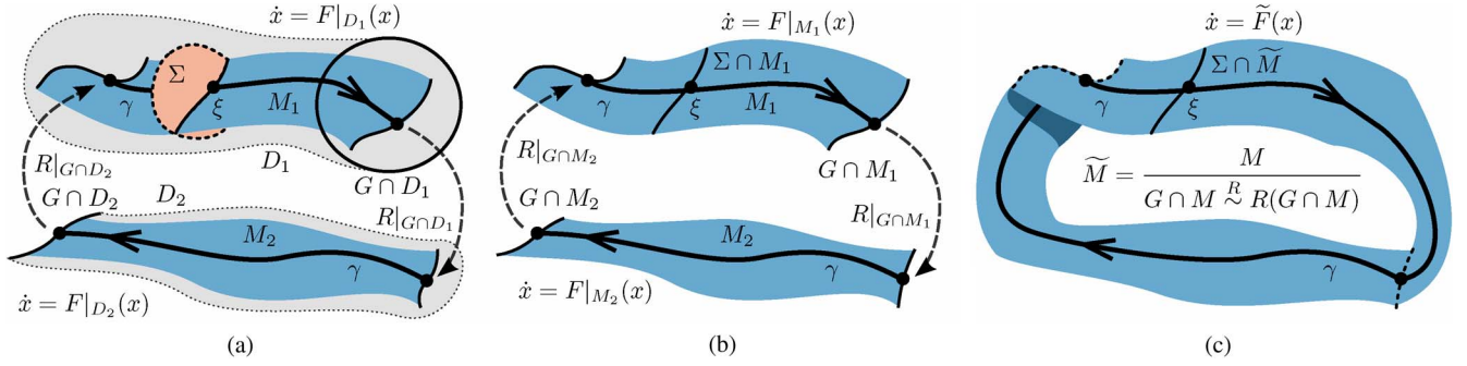
Fig. 2. (a) Applying Theorem 1 (Exact Reduction) to a hybrid dynamical system H = (D, F, G, R) containing a periodic orbit \gamma with associated Poincaré map P : U \rightarrow \Sigma yields an invariant subsystem M = \coprod_{j \in J} M_j ; nearby trajectories contract to M in finite time. (b) The subsystem may be extracted to yield a hybrid dynamical system H|_M . (c) The hybrid system H|_M may subsequently be smoothed via Theorem 3 (Smoothing) to yield a continuous-time dynamical system (\tilde{M}, \tilde{F}) . Application of Theorem 3 to the subsystem from Theorem 2 (Approximate Reduction) is illustrated by replacing H|_M with H|_{M^\varepsilon} . (a) H = (D, F, G, R) ; (b) H|_M = (M, F|_M, G \cap M, R|_{G \cap M}) ; (c) (\tilde{M}, \tilde{F}) .
