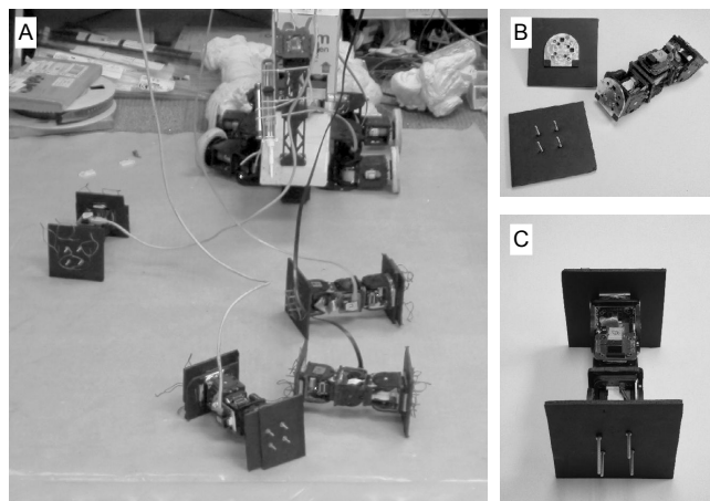
Fig. 4. Four clusters deploy from the synthesizer cart (A). Each cluster comprises three CKBot modules attached to foam interface plates via magnetically locking plates (B). Each cluster is a small mobile unit (C) capable of moving back and forth, rotating, and flipping to either side. In experiments clusters also had a nylon splatter shield cut from a shopping bag (not shown here; see videos)
