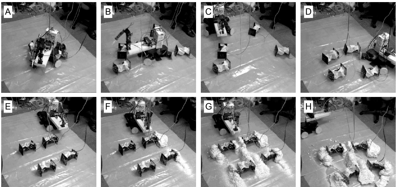
Fig. 5. Steps in forming and moving the a foam quadruped robot. We drove the synthesizer cart (A) and used it to deploy (B) four 3-module clusters (fig. 4). Using the clusters' ability to move and the cart's ability for pushing them, we aligned the clusters in a rectangular formation (B-D). We commanded the clusters to flip on their side so that joint axes are aligned appropriately for a quadruped (E) and then sprayed foam to form feet and a body (F,G). Once the foam hardened, the newly formed quadruped broke free of the ground and executed a breast-stroke like (symmetric) gait (H)
