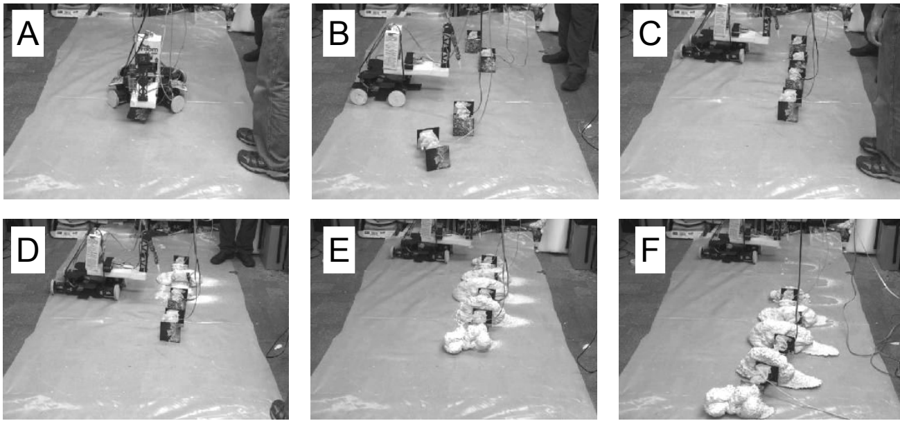
Fig. 6. Steps in forming and moving a foam snake robot. We activated the synthesizer cart (A) and used it to deploy four 3-module clusters (B). Using the clusters' ability to move and the cart's ability for pushing them, we aligned the clusters in a straight line (C) and poured foam between consecutive clusters bonding them (D). Once the foam expanded and hardened (E), we used gait commands to the newly formed "foam-snake" to cause it to move in both inchworm (F) and side-winding gaits.
