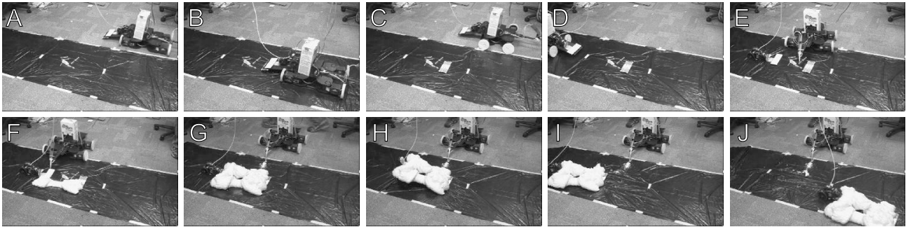
Fig. 3. Hazardous material needs to be removed from the floor (A). We drove the synthesizer cart to deploy the skid plate (B,C) and wheel arm (D,E). A foam plate sprayed from the robot captures the hazardous waste and provides a body for the removal robot (F,G). The wheel-arm uses the magnetic plates to situate under the plate (H) and drive the material away (I,J).
