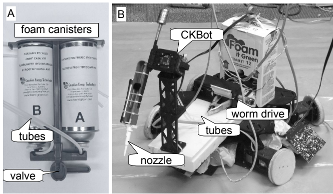
Fig. 1. Foam synthesizer system. A Two part foam with flow valve. B Foam system on a 4-wheel CKbot mobile base with nozzle mounted on an arm.
